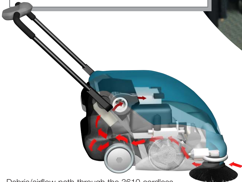
Debris/airflow path through the 3610 cordless vacuum/sweeper.
